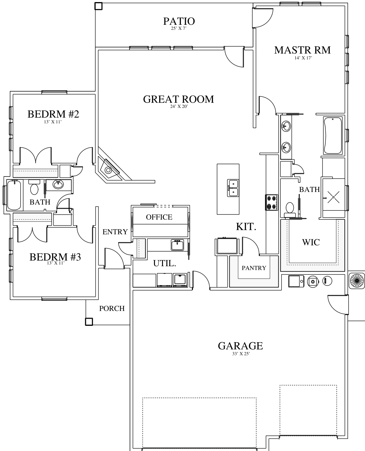
FLOOR PLAN 54' X 71'
